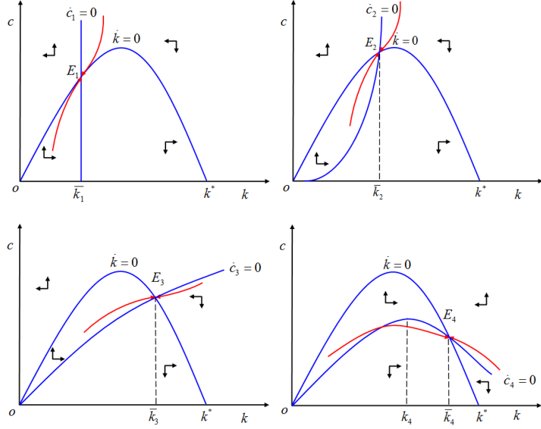
FIG. 1. The four cases a (top left), b (top right), c (bottom left), and d (bottom right) by the phase plane method
